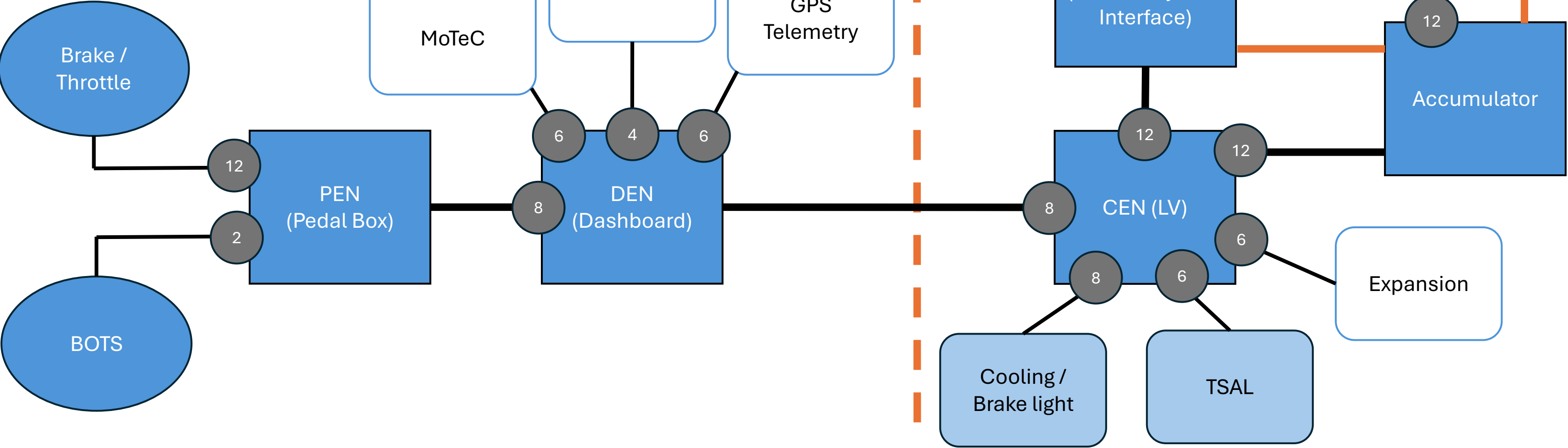
NU25 Electrical Topology
